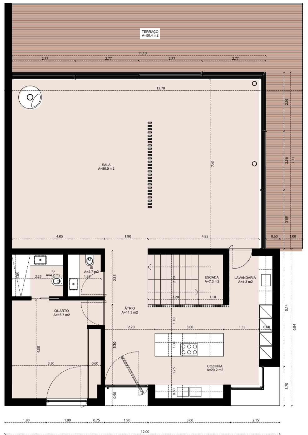
Ground floor | R/C
